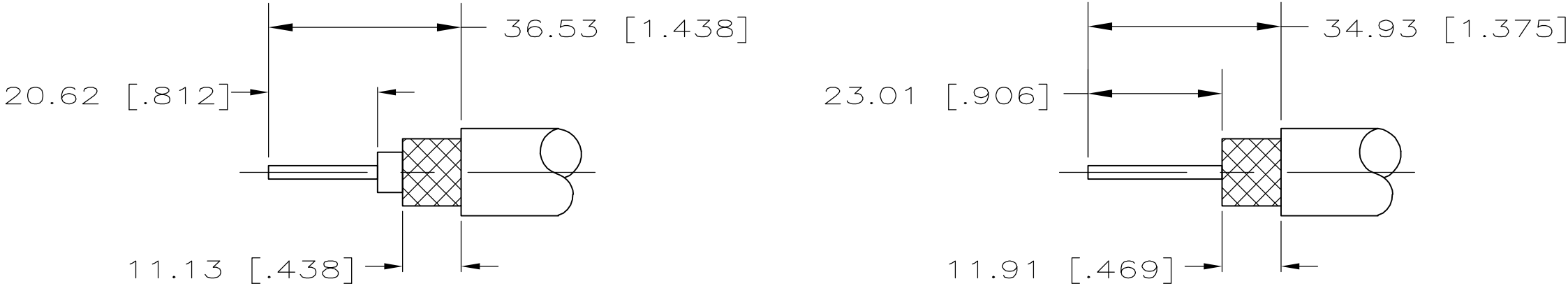
DETAIL A DETAIL B RECOMMENDED STRIP LENGTH
