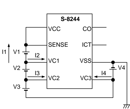
Test Circuit 1
