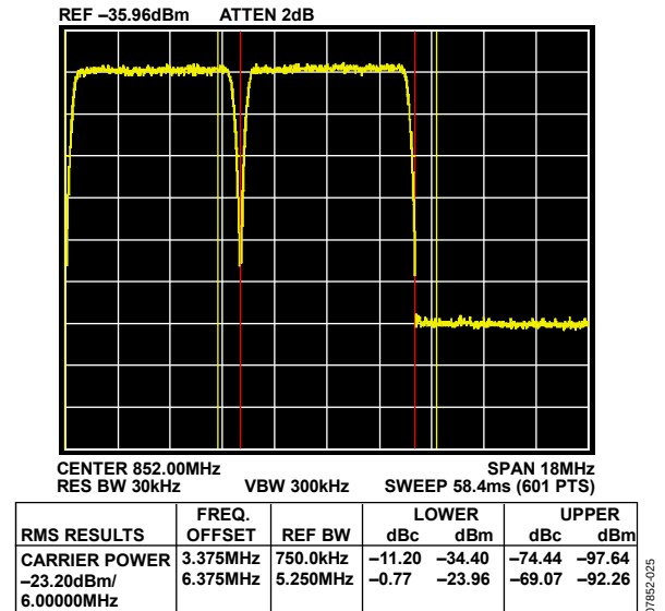
Figure 49. Zoomed 4-Channel QAM ACLR, f_{OUT} = 840 MHz, Temperature = 25°C, Sum Scale = 20, Full-Scale Current = 25 mA, Span = 18 MHz, Channel 4
