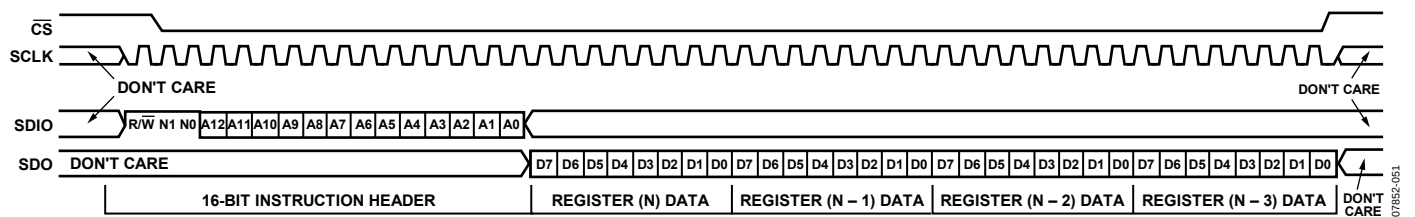
Figure 65. Serial Control Port Read—MSB First, 16-Bit Instruction, Four Bytes of Data
