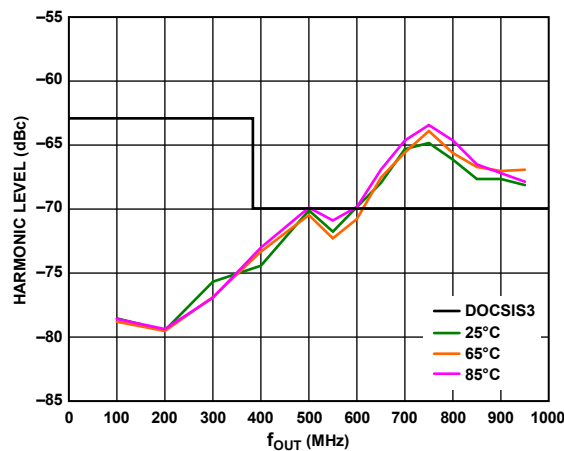
Figure 28. Third-Order Harmonic Performance vs. f_{OUT} over Temperature, 2-Channel QAM, f_{DAC} = 2.3 GHz, Full-Scale Current = 25 mA, Sum Scale = 32 (DOCSIS SPEC Is -70 dBc; Harmonic Exception Is -63 dBc)
