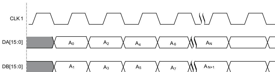
Figure 38. HALF RATE BUS MODE (Dual Clock Mode)
