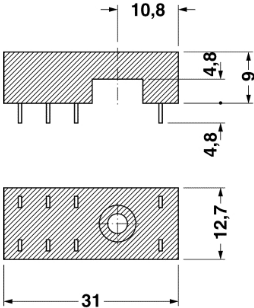
Dimensioned drawing
