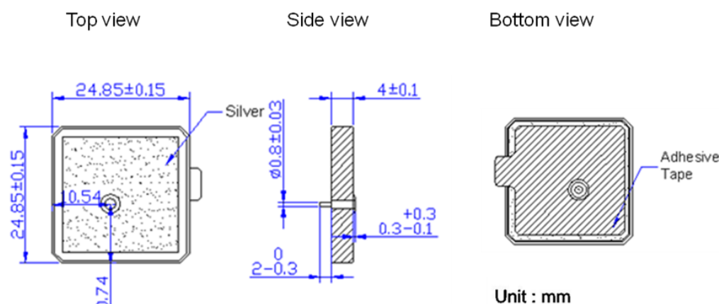
Fig. 1 Mechanical data
