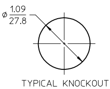
TYPICAL KNOCKOUT
