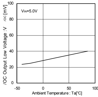
Fig.16 /OC output low voltage
