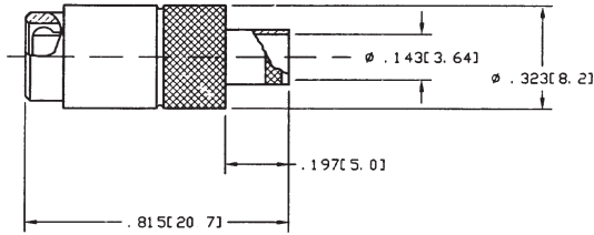
Straight Push-Pull Plugs Solder to Body 102-799-41 for .141 (3.6mm) SR RG 402 102-799-85 for .085 (2.2mm) SR RG 405
