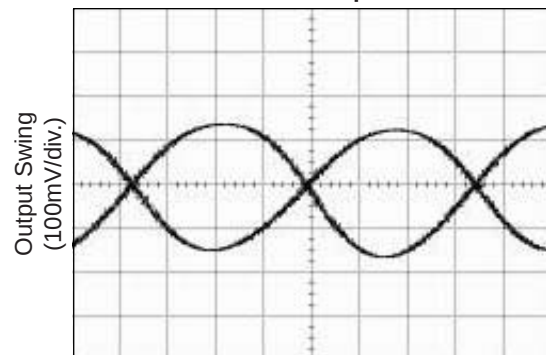
7GHz Output
