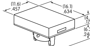
AT4021 Rectangular
