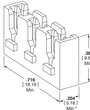
Cavity Specification 1601440
