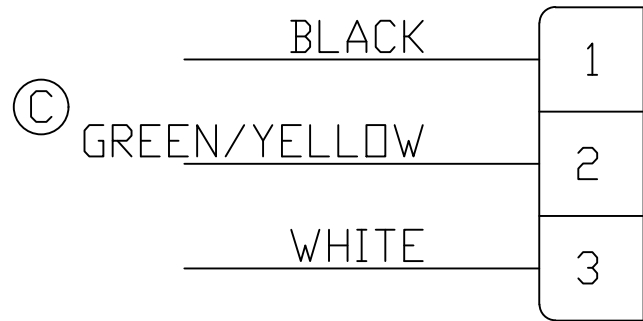
WIRING DIAGRAM
