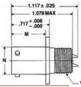
LJT01T-XX-XXX (MS20027T)
