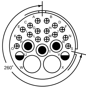
260° Rotation of 32-6
