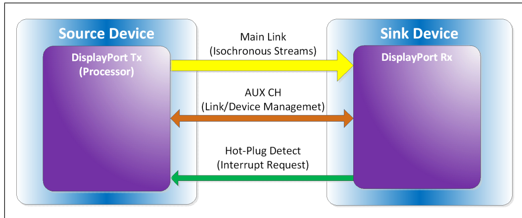
Figure 2-6. DisplayPort* Overview
