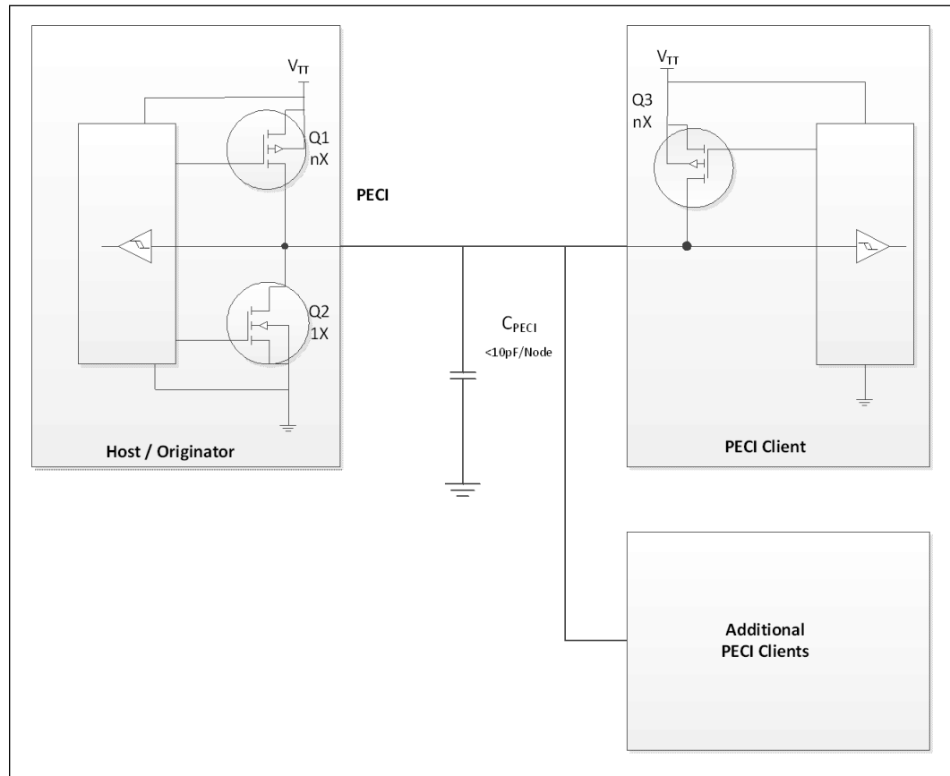
Figure 2-8. Example for PECl Host-Clients Connection
