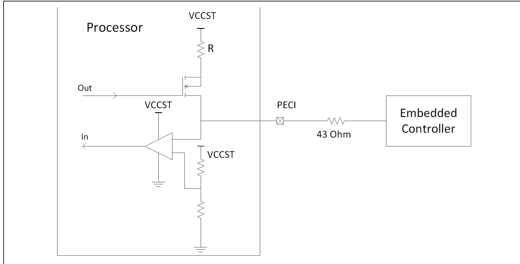
Figure 2-9. Example for PECE EC Connection
