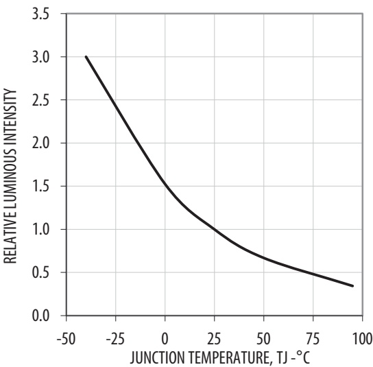
Figure 7: Relative Intensity vs. Temperature
