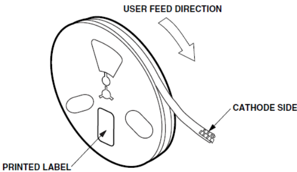
Figure 12: Reel Orientation
