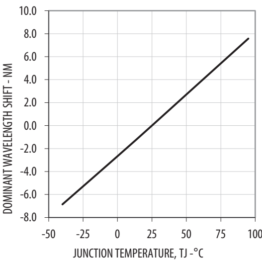
Figure 9: Wavelength Shift vs. Temperature
