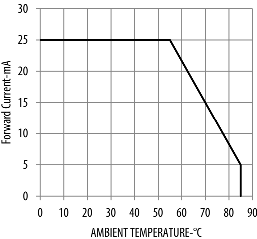
Figure 10: Derating Curve
