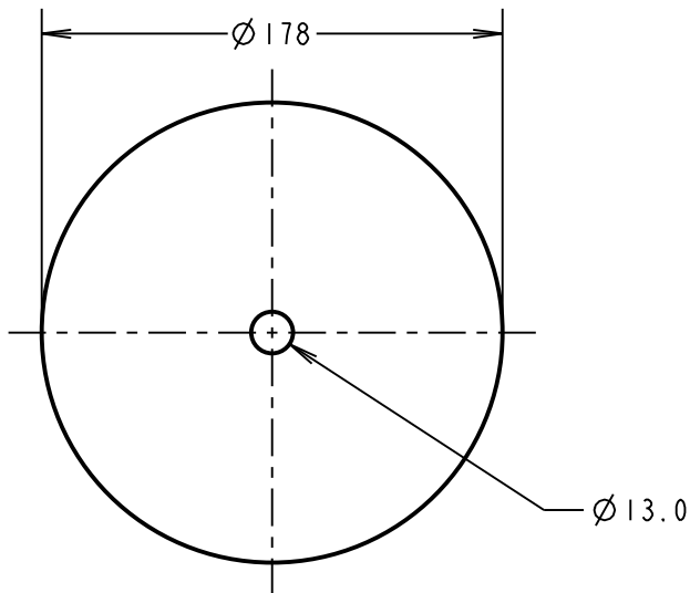
REEL DETAILS
