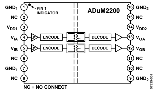
Figure 1. ADuM2200
