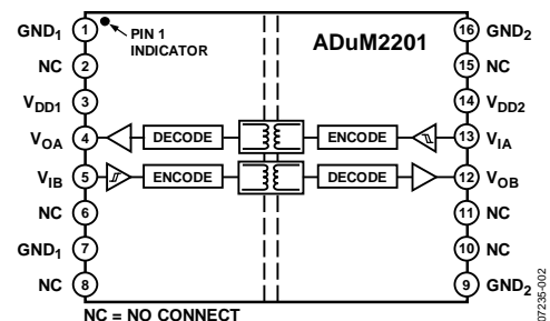
Figure 2. ADuM2201
