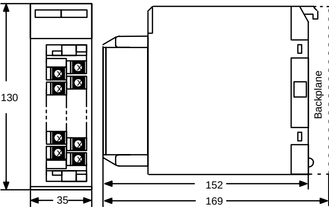
19-terminal Terminal Block (Extended B-shape I/O Units)
