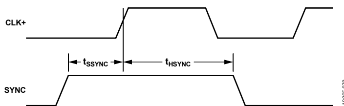
Figure 8. SYNC Input Timing Requirements
