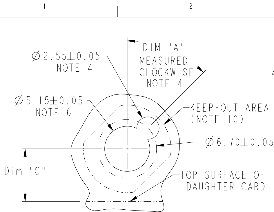
RECOMMENDED PCB LAYOUT (DRILLING) NOTES 4, 6, & 7 SCALE 4:1
