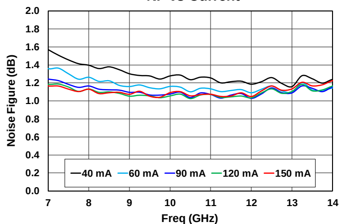
NF vs Current
