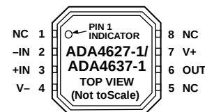
NOTES 1. NC = NO CONNECT. 2. IT IS RECOMMENDED THAT THE EXPOSED PAD BE CONNECTED TO V-. Figure 3. 8-Lead LFCSP_VD (CP-8-2)
