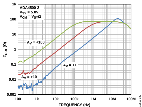
Figure 34. Closed Loop Output Impedance ( Z_{OUT} ) vs. Frequency, V_{SV} = 5.0\text{ V}
