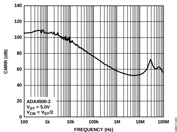
Figure 32. CMRR vs. Frequency, V_{SV} = 5.0\text{ V}
