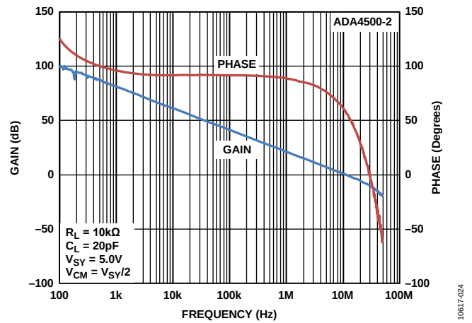
Figure 27. Open-Loop Gain and Phase vs. Frequency, V_{SV} = 5.0\text{ V}
