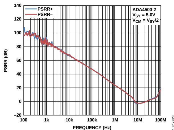
Figure 33. PSRR vs. Frequency, V_{SV} = 5.0\text{ V}
