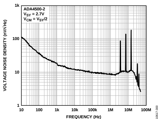
Figure 50. Voltage Noise Density vs. Frequency, V_{SV} = 2.7\text{V} (10 Hz to 100 MHz)
