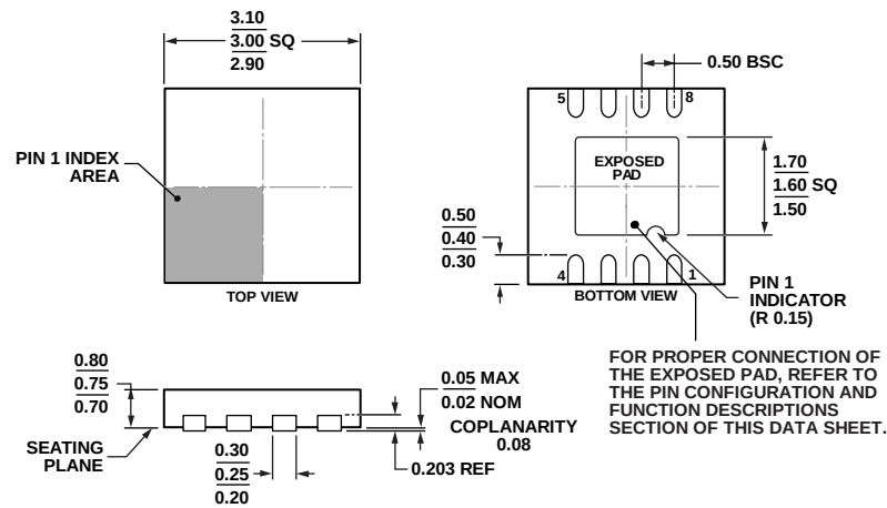
Figure 67. 8-Lead Lead Frame Chip Scale Package [LFCSP_WD] 3 mm x 3 mm Body, Very, Very Thin, Dual Lead (CP-8-12) Dimensions shown in millimeters
