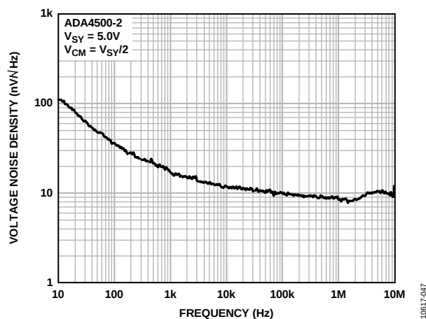
Figure 52. Voltage Noise Density vs. Frequency, V_{SV} = 5.0\text{V} (10 Hz to 10 MHz)
