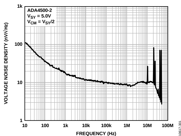
Figure 53. Voltage Noise Density vs. Frequency, V_{SV} = 5.0\text{V} (10 Hz to 100 MHz)
