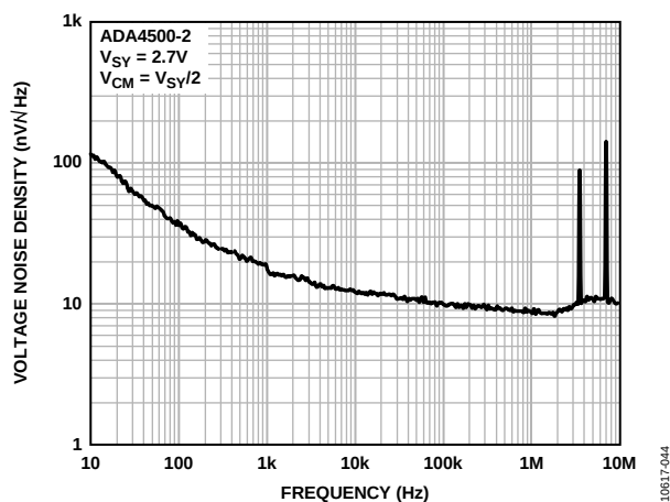
Figure 49. Voltage Noise Density vs. Frequency, V_{SV} = 2.7\text{V} (10 Hz to 10 MHz)
