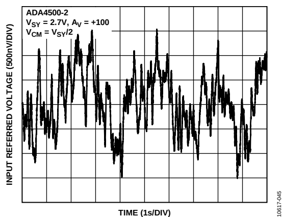
Figure 51. 0.1 to 10 Hz Noise, V_{SV} = 2.7\text{V}
