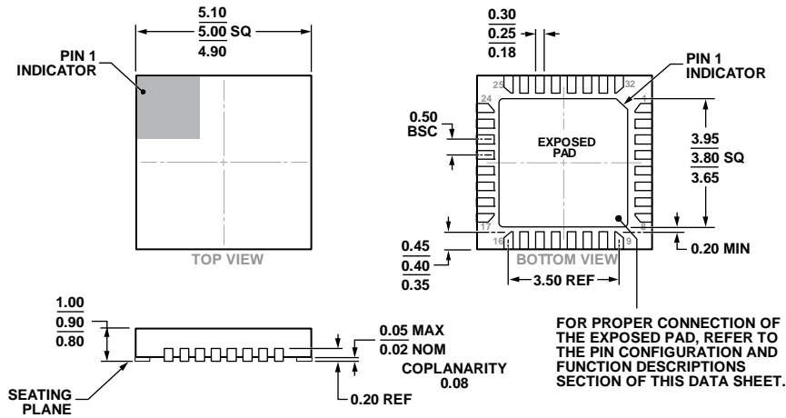
COMPLIANT TO JEDEC STANDARDS MO-220-VHDD-4. Figure 18. 32-Lead Lead Frame Chip Scale Package [LFCSP] 5 mm x 5 mm Body and 0.90 mm Package Height (HCP-32-3) Dimensions shown in millimeters
