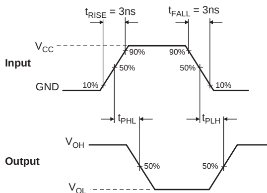
Figure 3. AC Waveforms
