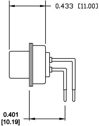
SIGNAL CONTACTS
