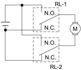
Test circuit
