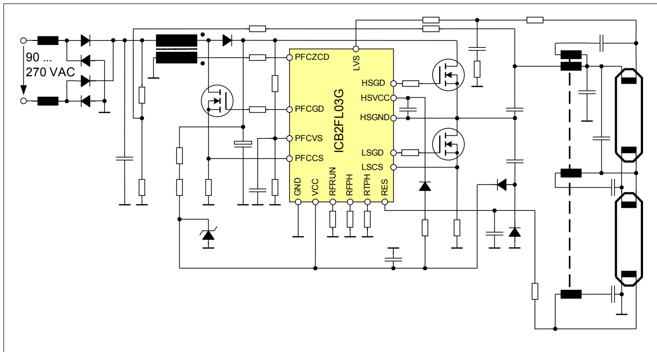
Figure 39 Application Circuit of Ballast for two Fluorescent Lamps Voltage Mode Preheating
