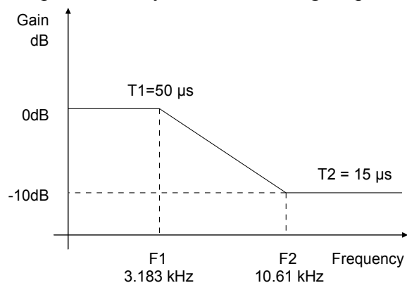
Figure 7. De-Emphasis Curve
