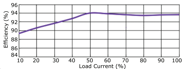
VX078012-500 Efficiency Curve Positive Output, Efficiency vs. Load Current (at Vin nominal)
