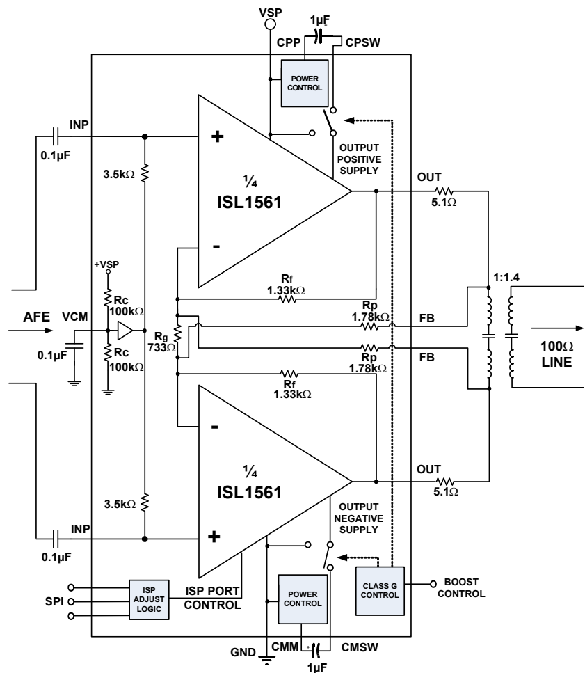
TYPICAL DIFFERENTIAL I/O LINE DRIVER (1 OF 2 PORTS)
