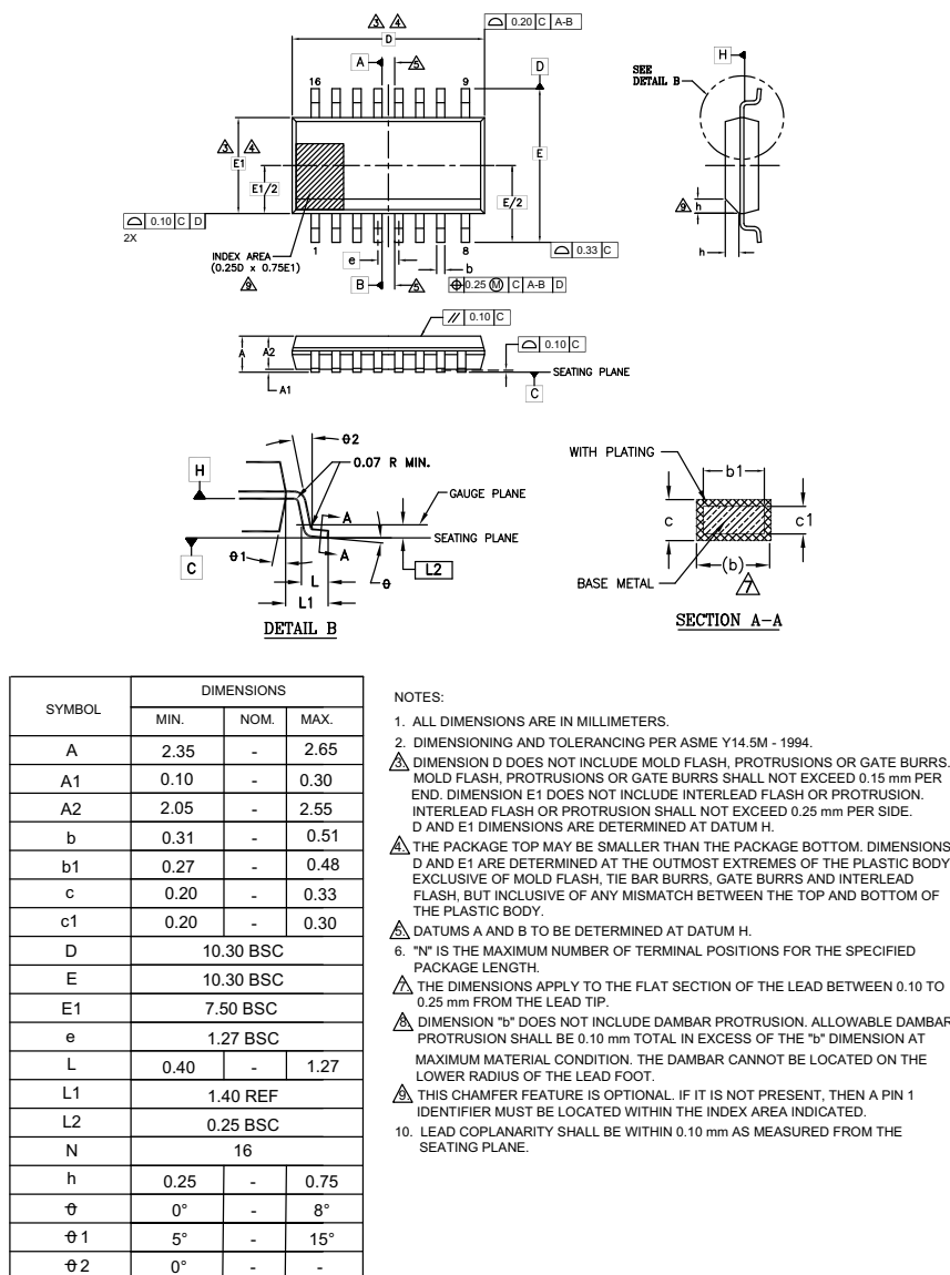
Figure 36. SOIC 16-Lead, 300-mil Body Width (SO3016)
