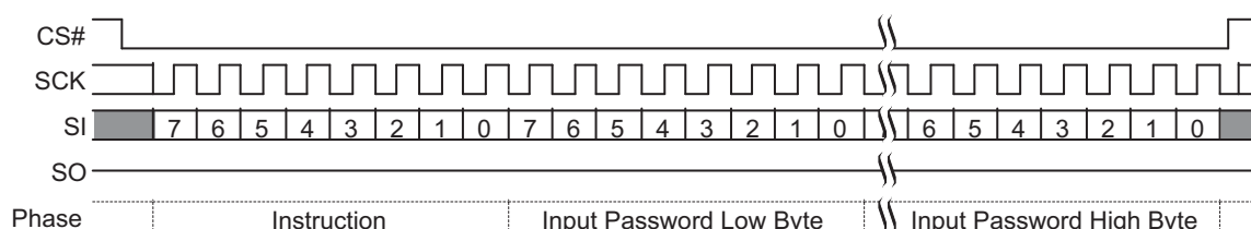
Figure 114. Password Unlock Command Sequence
