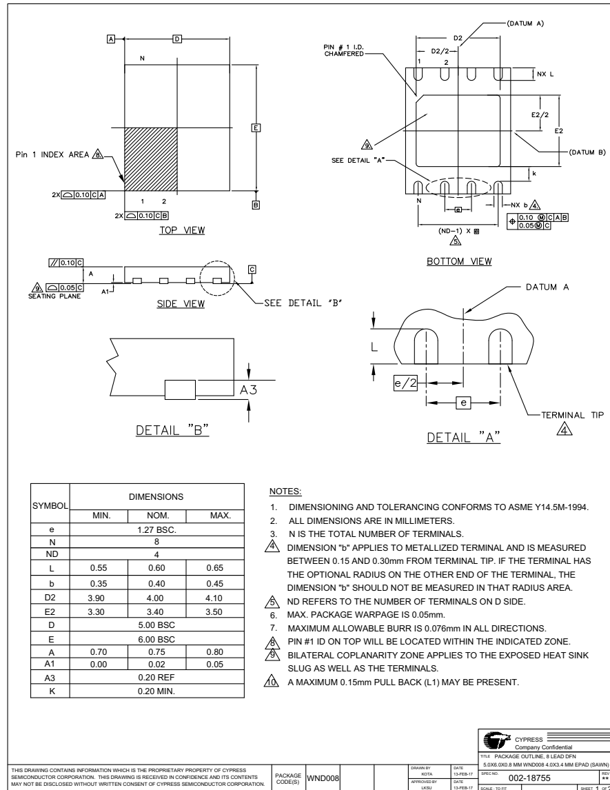
Figure 40. WSON 8-Contact 6x5 mm Leadless (WND008)
