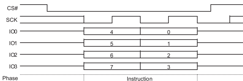
Figure 116. Software Reset Command Sequence QPI Mode
