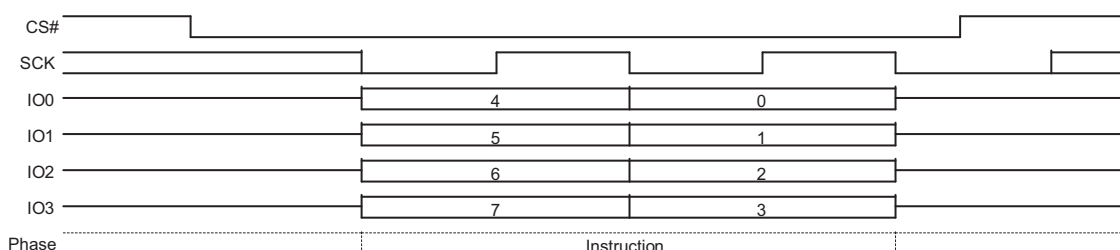
Figure 93. Bulk Erase Command Sequence QPI Mode
