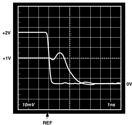
TPC 57. AD8036 Clamp Overdrive (2 \times ) Recovery
