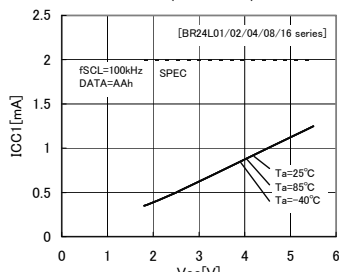
Fig.12 Current consumption at WRITE action ICC1 ( f_{SCL}=100\text{kHz} )
