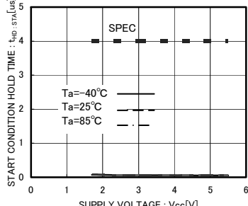
Fig.16 Start Condition Hold Time t HD:STA
