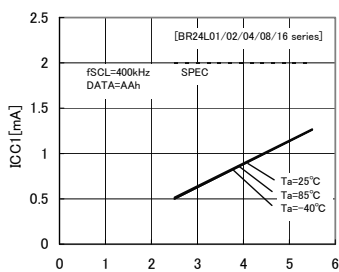
Fig.9 Current consumption at WRITE action ICC1 ( f_{SCL}=400\text{kHz} )
