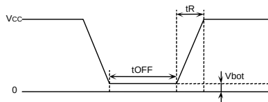
Fig.56 Rise waveform diagram
