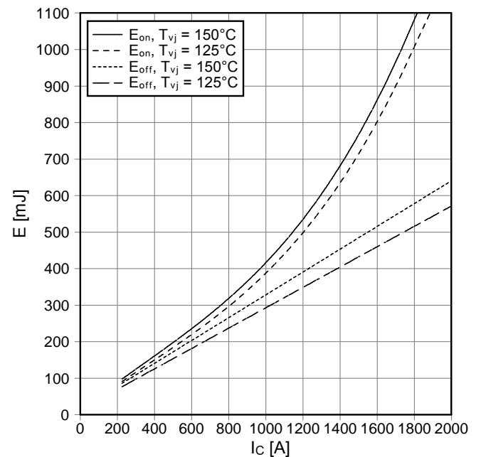
Schaltverluste IGBT-Wechselr. (typisch) switching losses IGBT-inverter (typical) E_{on} = f(I_C), E_{off} = f(I_C) V_{GE} = \pm 15\text{ V}, R_{Gon} = 1.2\ \Omega, R_{Goff} = 1.8\ \Omega, V_{CE} = 900\text{ V}
