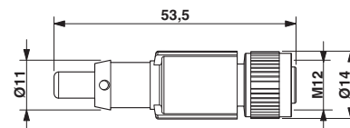
Dimensional drawing
