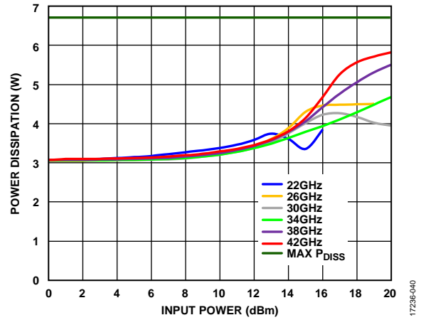
Figure 38. Power Dissipation (P DISS ) vs. Input Power, T A = 85°C
