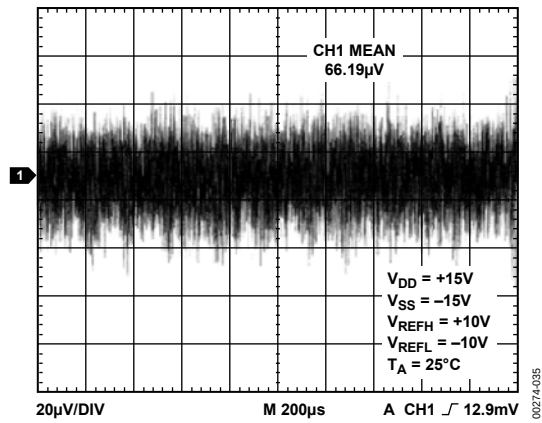
Figure 34. Broadband Noise
