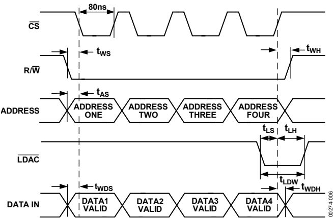
Figure 6. Double-Buffer Mode
