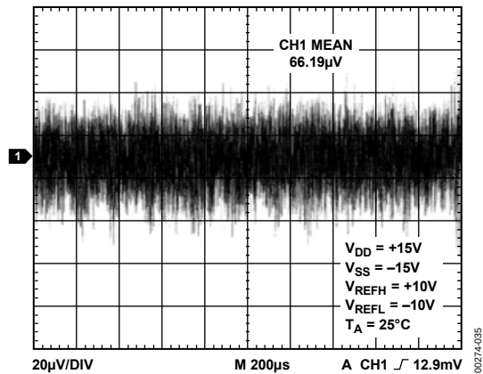
Figure 34. Broadband Noise
