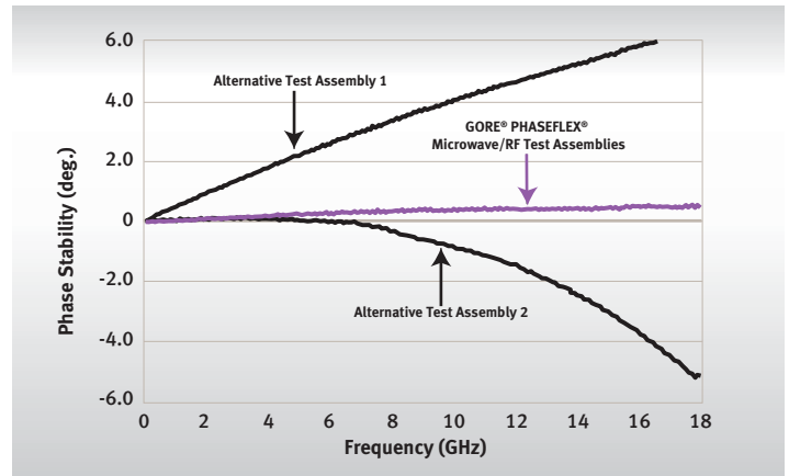
FIGURE 4: PHASE STABILITY WITH FLEXURE OF NEW CABLES
