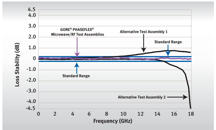
FIGURE 5: LOSS STABILITY OVER TIME
