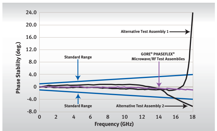
FIGURE 6: PHASE STABILITY OVER TIME
