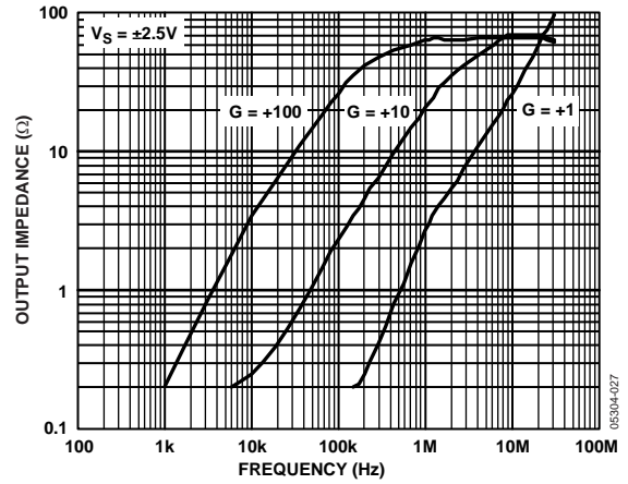
Figure 30. Output Impedance vs. Frequency
