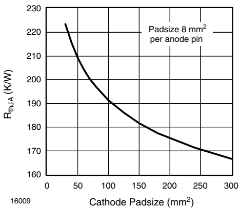
16009 Fig. 4 - Thermal Resistance Junction Ambient vs. Cathode Padsizes
